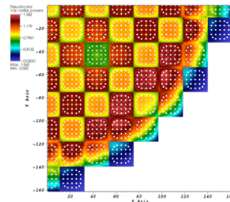
Figure 5. Reference CE Monte Carlo power distribution for AP-1000 reactor
