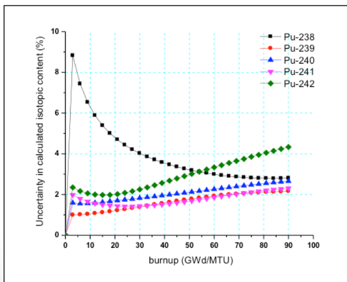
Figure 10. Uncertainty in plutonium isotopics in LWR depletion
