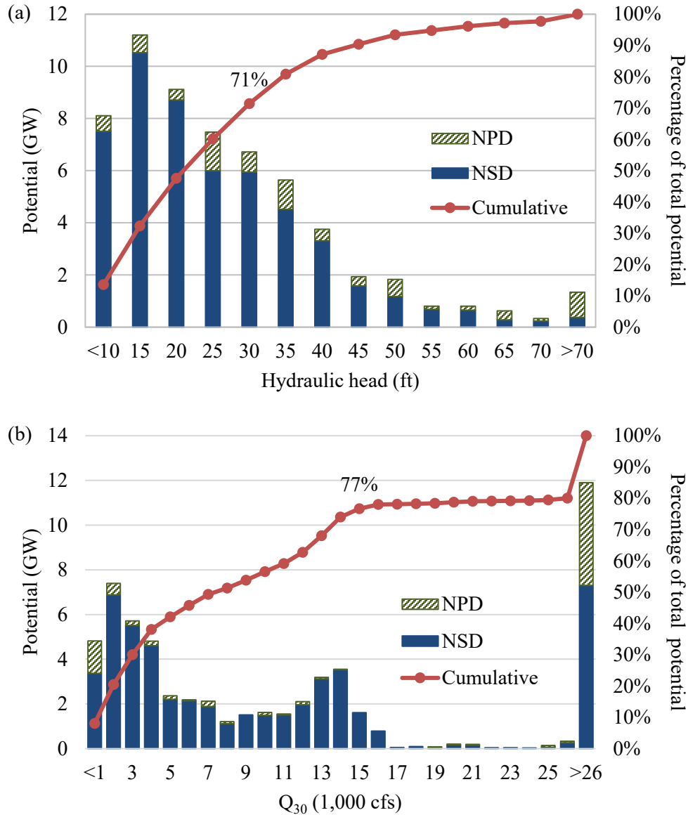
Figure 3. Histogram of NSD and NPD development potential in the United States (Hadjerioua, Wei, and Kao 2012; Kao et al. 2014) organized by (a) head and (b) Q 30 flow (watershed average 30% flow exceedance). Only includes sites with >1 MW of potential capacity and available flow and head data. The red dotted lines indicate the percentage of total cumulative potential (i.e., 59.7 GW total: 51.5 GW of NSD and 8.2 GW of NPD) for a given head or flow. The data labels highlight head and flow points that are relevant for the testing criteria in Section 5.2.2.
