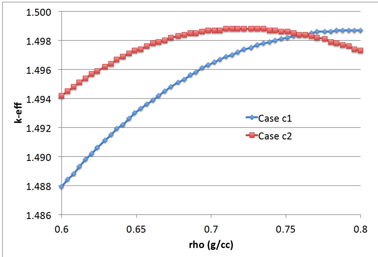
Figure 6.7.6. Dependency of lambda (k-eff) on coolant density for sample problem 2
