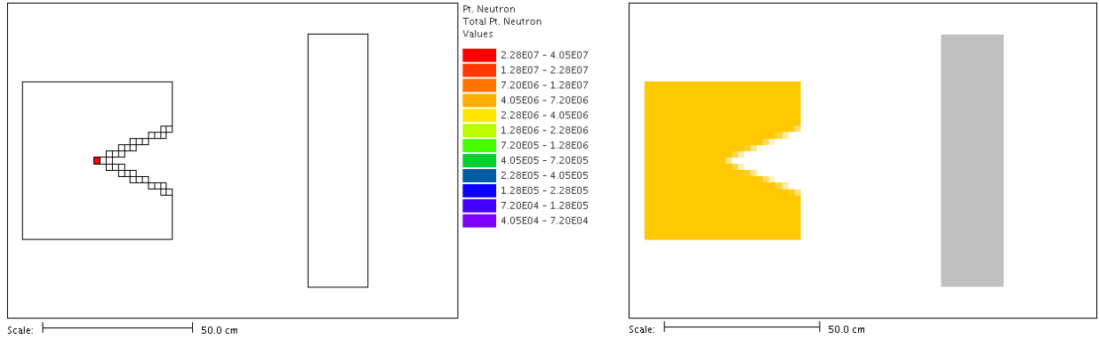
Figure 4.1.C.5. Forward Denovo source (left) and mesh geometry (right).
