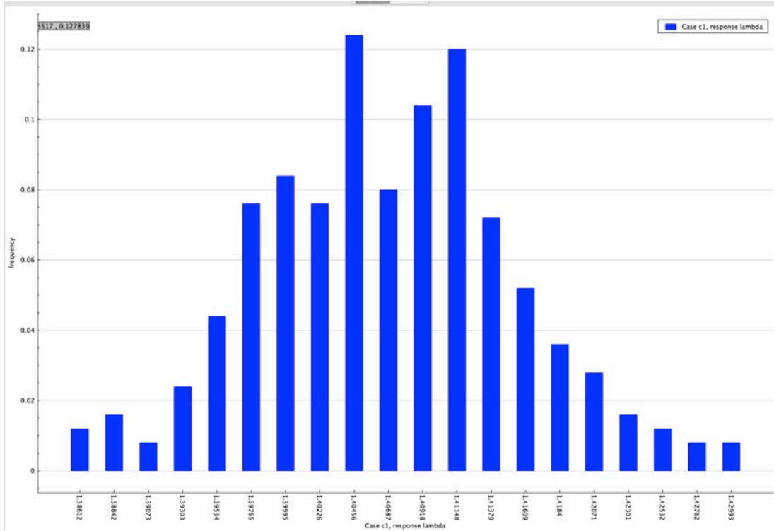
Figure 6.7.5. Distribution of lambda (k-eff) obtained from sample problem 1
